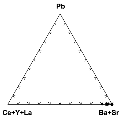
Figura 7: Diagrama ternario Ce+Y+La vs. Ba+Sr vs. Pb .
