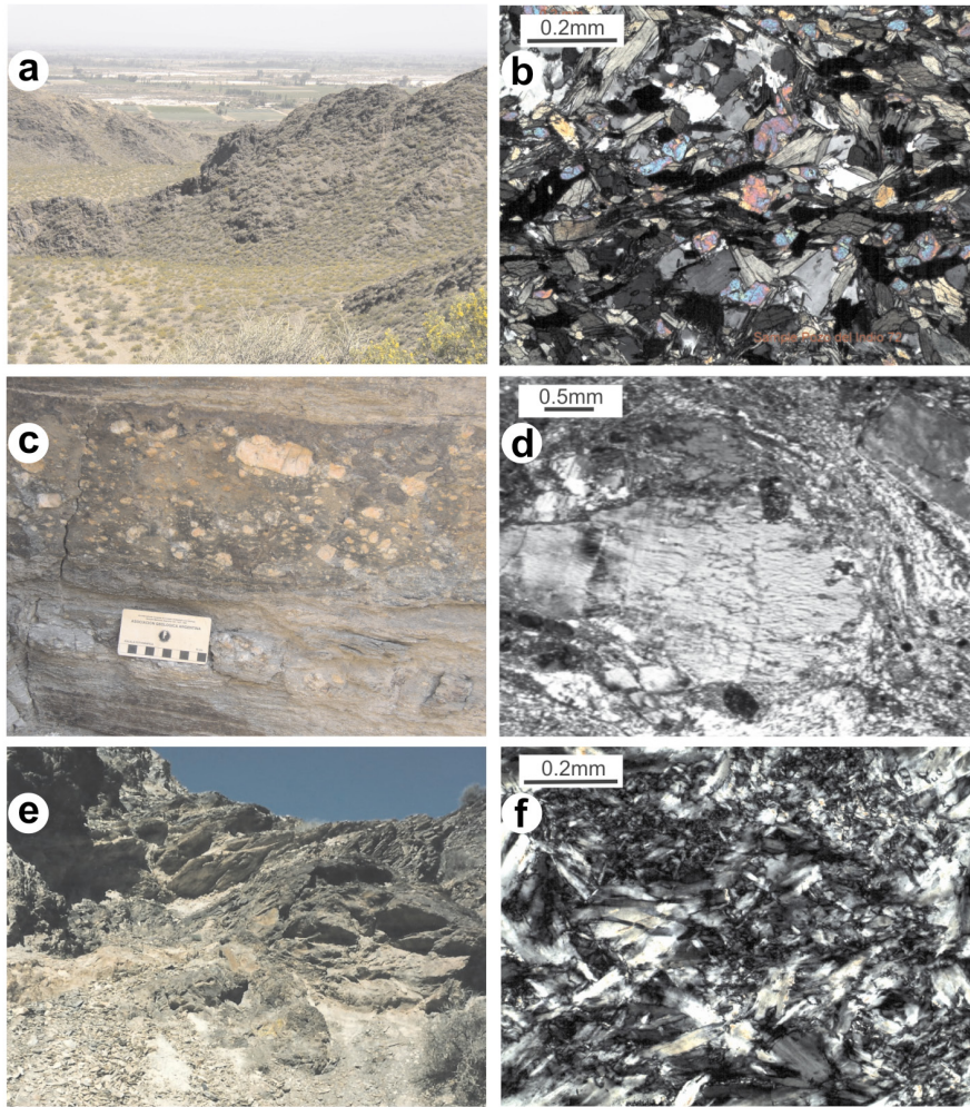
Figure 5: Outcrop views and the corresponding photomicrographs of some representative rock types analyzed in Table 1. (A), (B), ... indicate sample locations shown in figure 1. a-b) Ep-chl-am schist (D). c-d) Augen orthogneiss (B). e-f) Serpentinite mainly composed of antigorite (A). All photomicrographs under crossed polars. Mineral abbreviations after Siivola and Schmid (2007).
