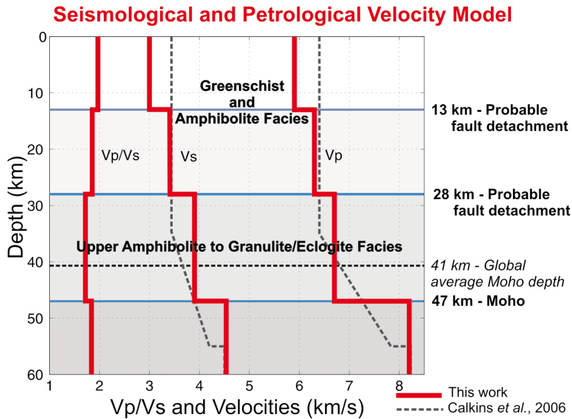
Figure 6: Proposed seismic and petrological crustal model for the southwest of the Sierra de Pie de Palo. For comparison a seismic model by Calkins et al. (2006) in the same region and the average Moho depth in continental regions by Christensen and Mooney (1995) are also shown.
