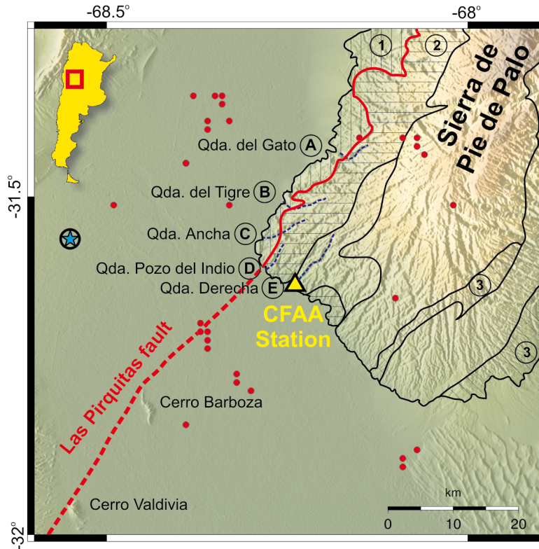
Figure 1: Region of study in the southwest of the Sierra de Pie de Palo. CFAA denotes the broadband seismic station used and the red (piercing point) dots, the incidence of coming teleseismic waves at 47 km depth (Moho depth estimation from Perarnau et al. 2010). Geology adapted from Chernicoff et al. (2009) and others therein. References: (1) Cauçete Group; (2) Pie de Palo Complex including the mafic-ultramafic belt (horizontal lines); (3) Difunta Correa Sequence. (A) to (E) indicate sample locations cited in figures 4 and 5.
