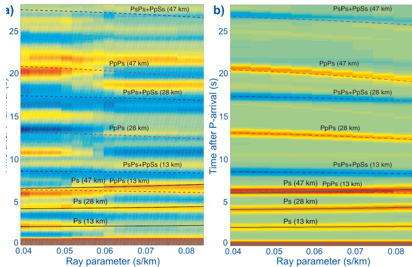
Figure 3: a) Observed receiver functions varying with epicentral distances (ray parameters). b) Synthetic receiver functions built for the crustal model constrained in this study (see Fig. 6). Note the good correlation between mid-crustal (13 km and 28 km depths) and the Moho (47 km) observed and predicted primary arrivals.
